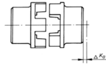
Axial misalignment
