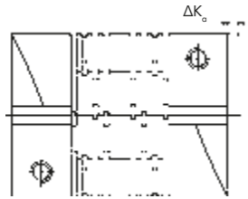
Axial misalignment
