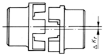
Radial misalignment
